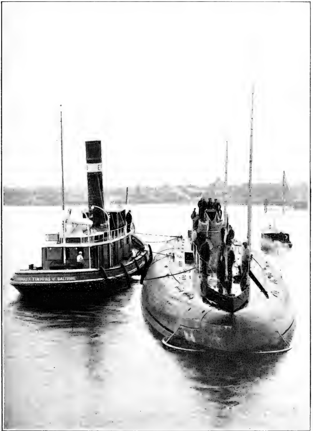
© Int. Film Serv. Looking More Like the Familiar Whale-Back Than Anything Else, the "Deutschland" Made Her Way into Baltimore to the Astonishment of the Entire World. She Is Three Hundred Feet Long and Therefore Smaller Than the Enormous Craft Which Rumor Had Taught Us To Expect
